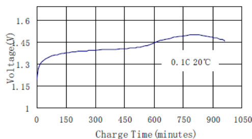
Typical Charge Characteristics
