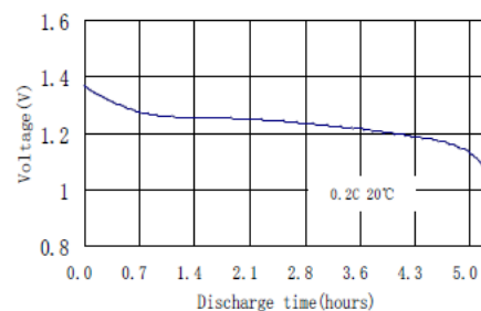
Discharge at low rate
