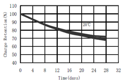
Charge Retention
