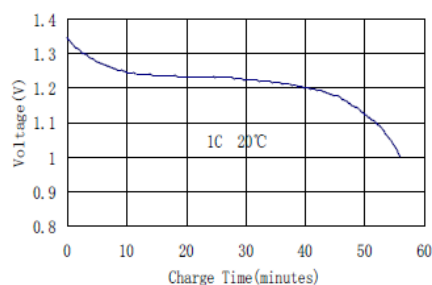
Typical Charge Characteristics
